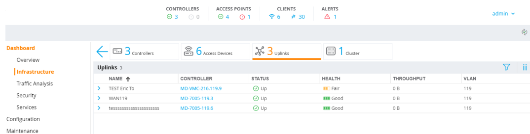
Figure 48 Uplinks Page
