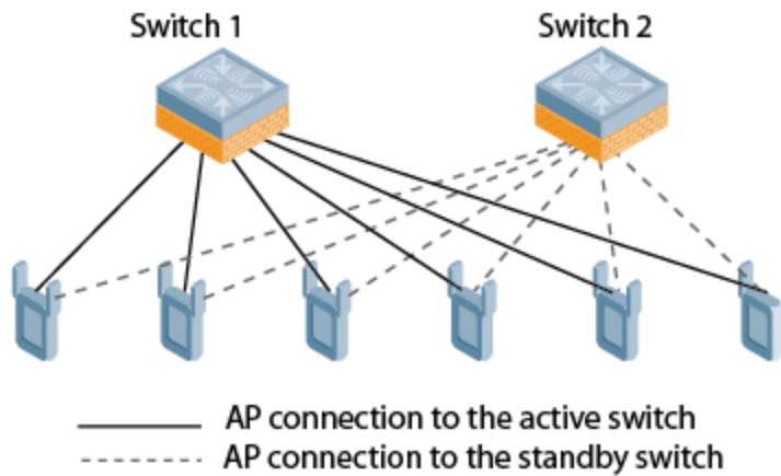
Figure 91 1:1 Active/Standby Deployment
