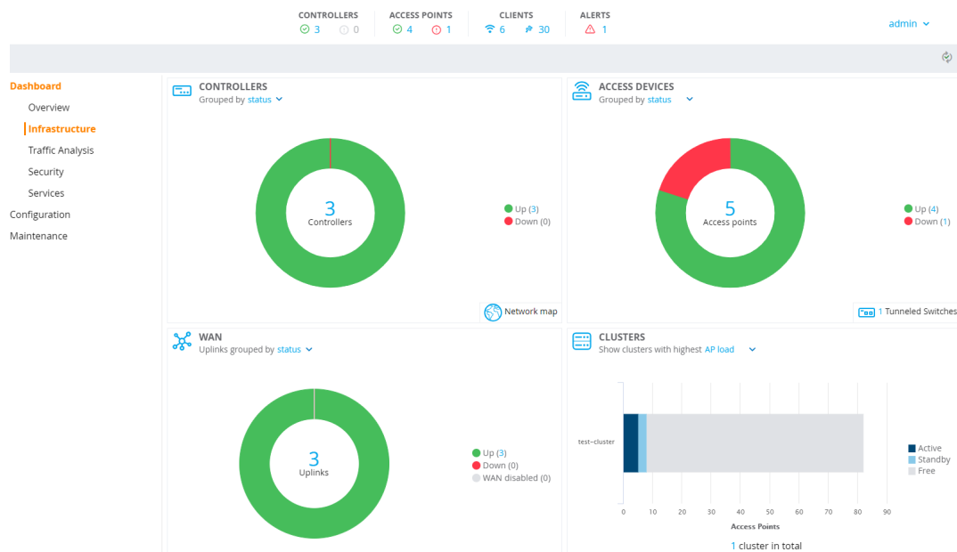
Figure 43 Infrastructure Page
