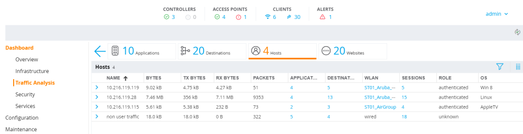
Figure 62 Hosts Page
