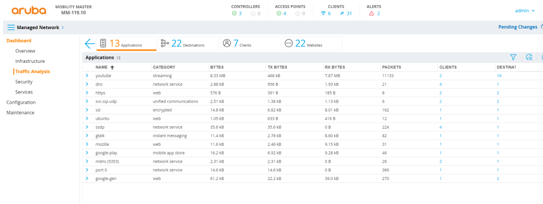
Figure 58 Applications Page
