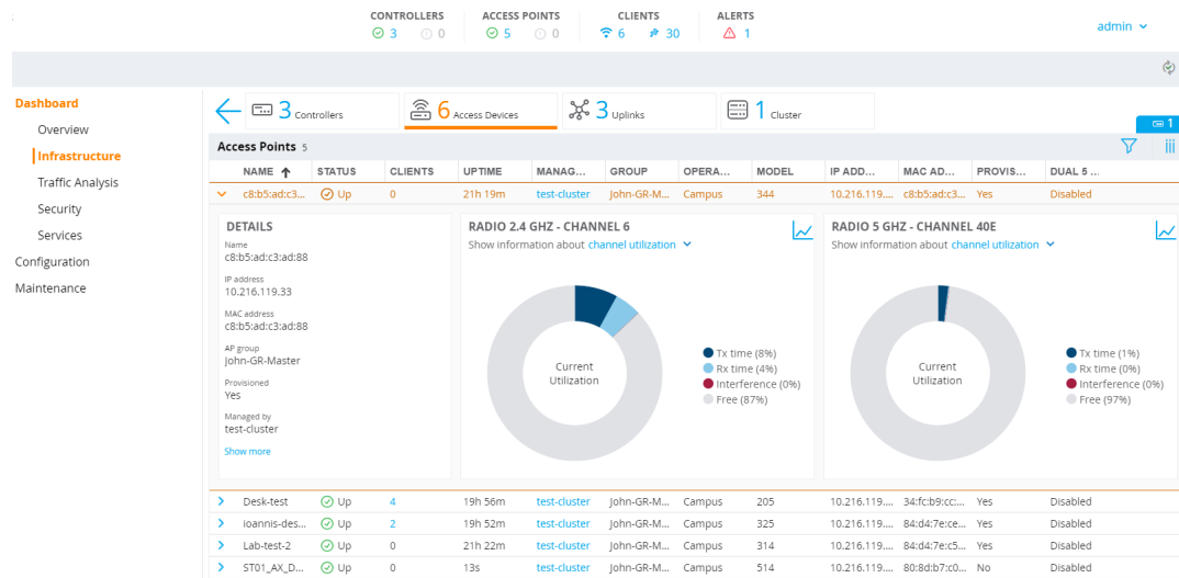
Figure 47 Details Page
