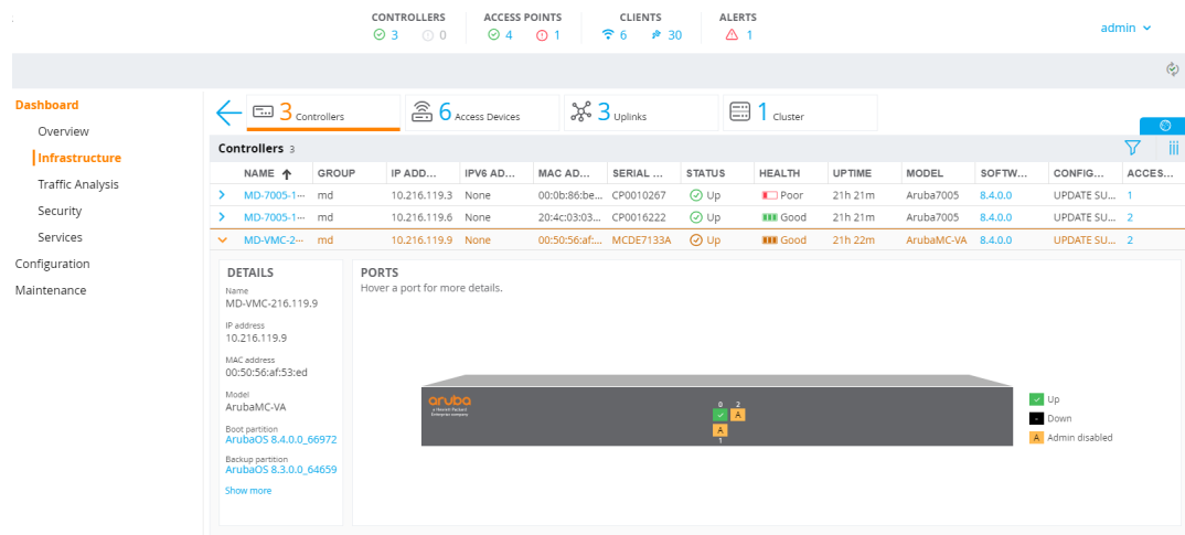
Figure 45 Details Page
