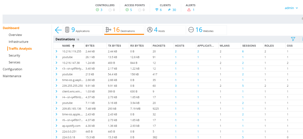
Figure 60 Destinations Page
