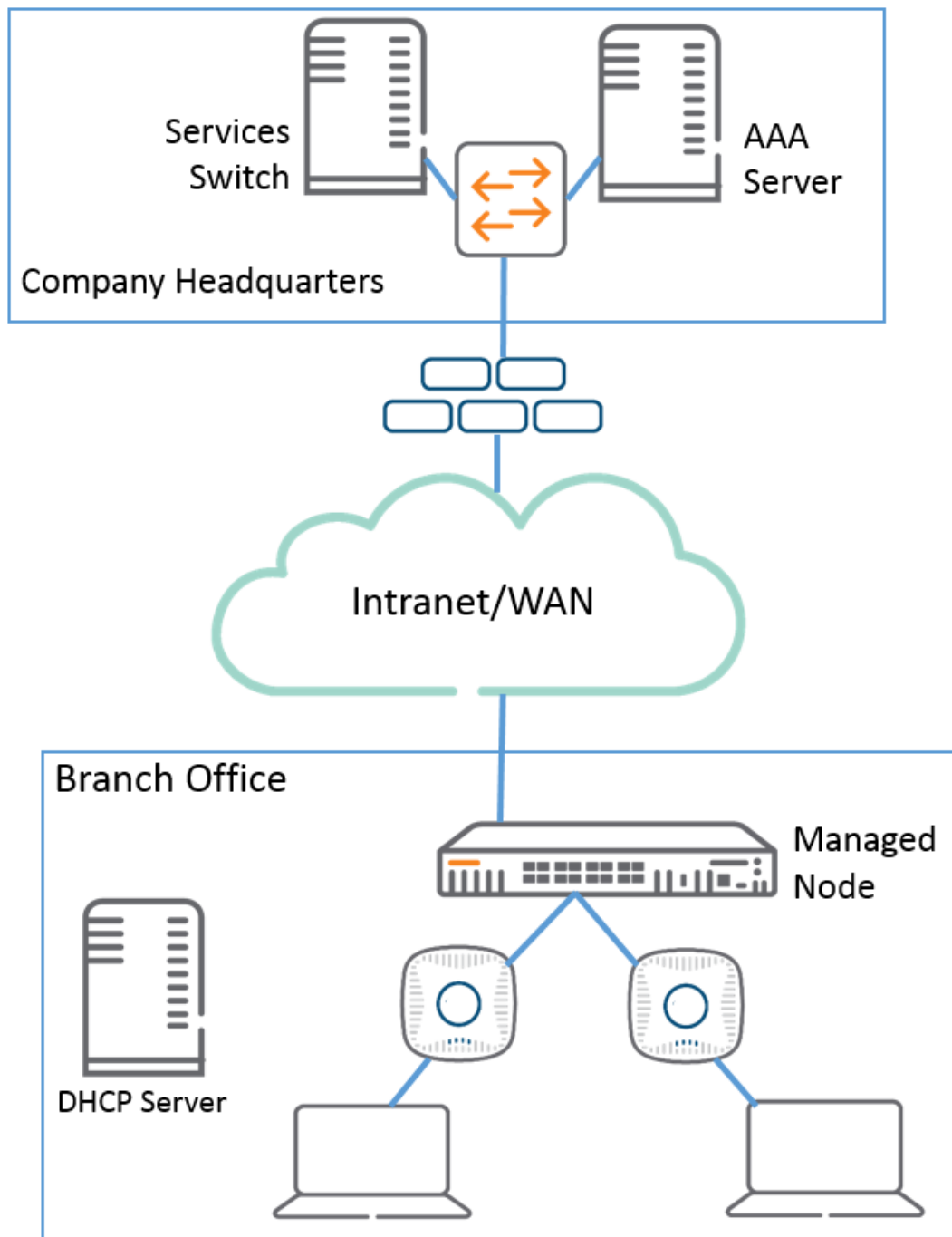
Figure 27 Managed Device Topology
