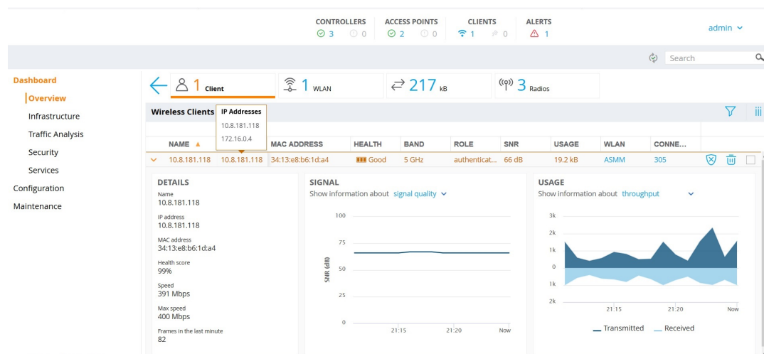
Figure 36 Details Page
