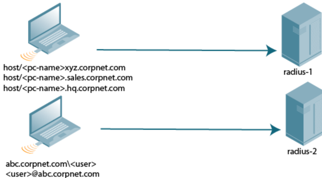
Figure 25 Server Group
