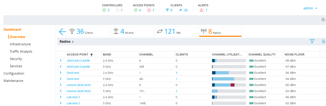
Figure 41 Radios Page
