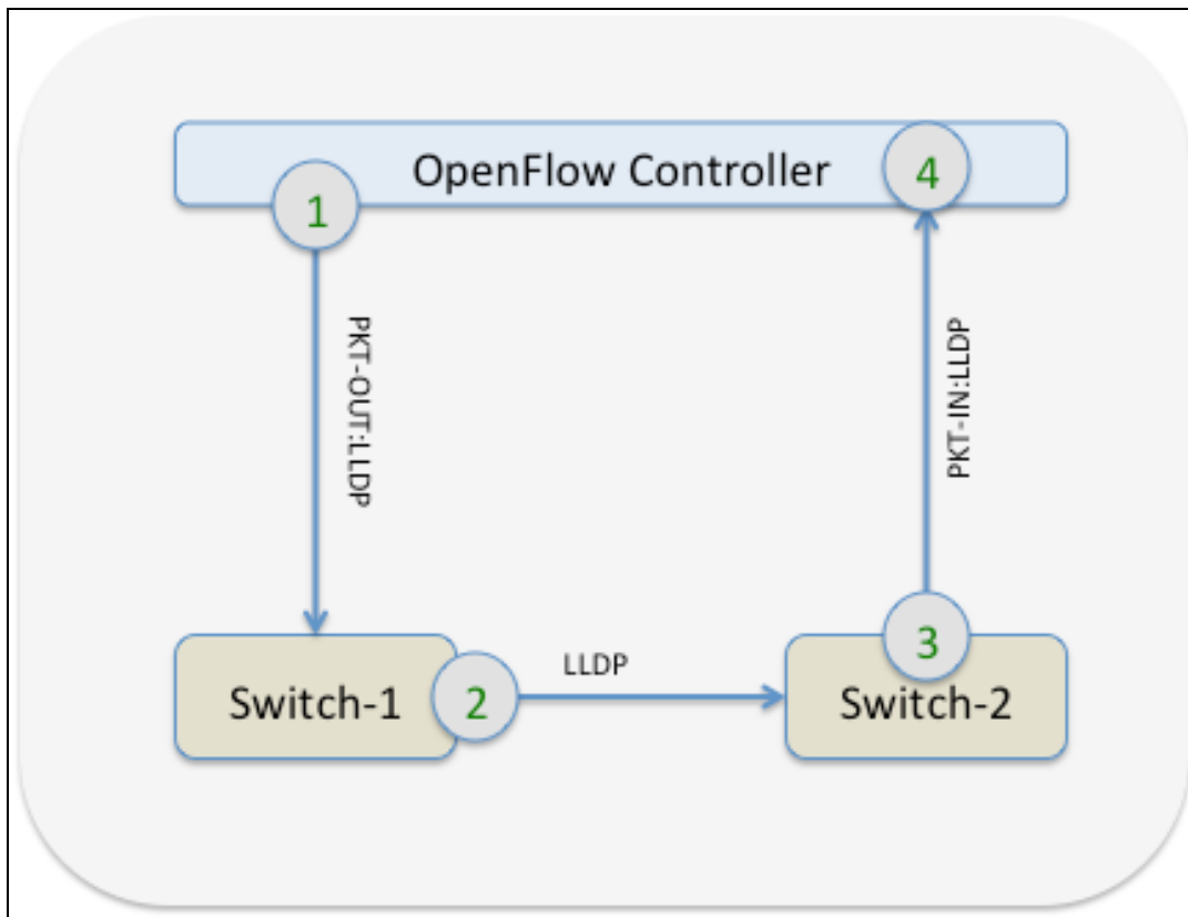
Figure 118 Topology Discovery
