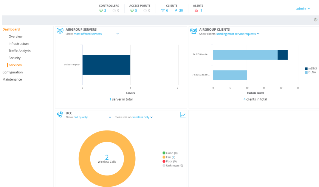
Figure 74 Services Page
