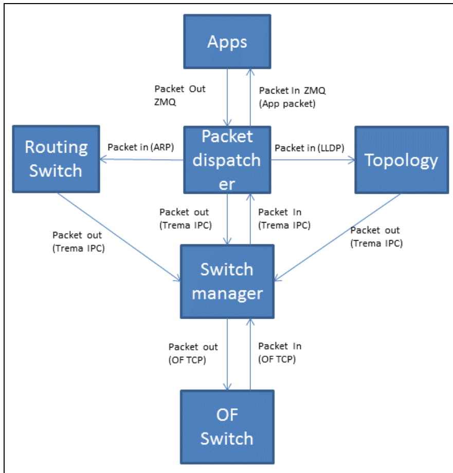
Figure 121 Packet Handling
