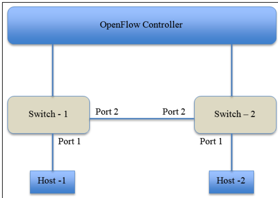
Figure 119 Host Discovery
