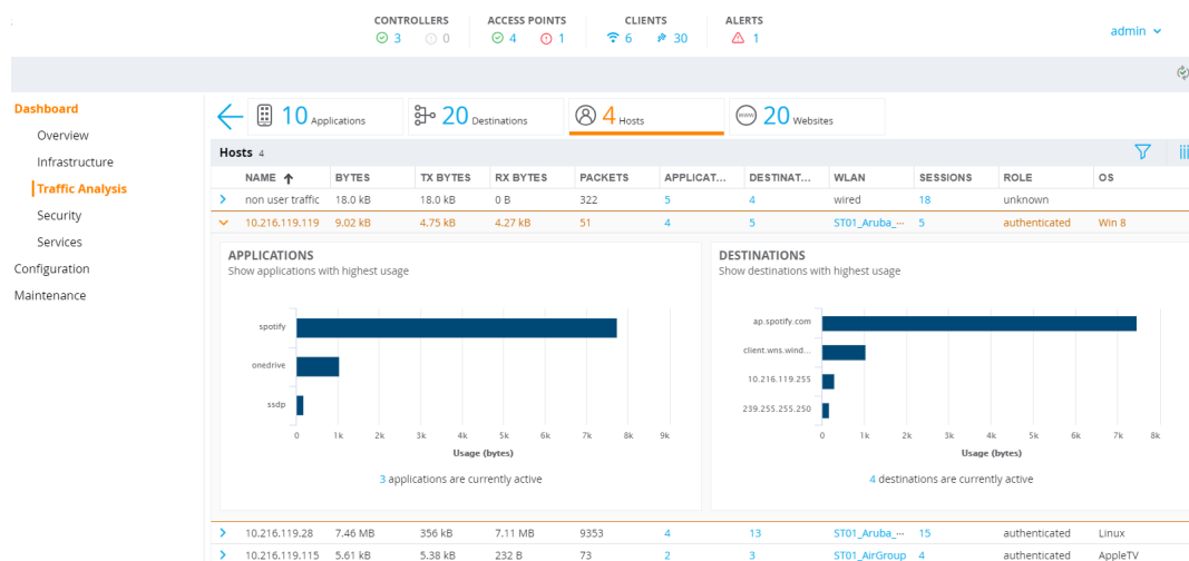
Figure 63 Details Page
