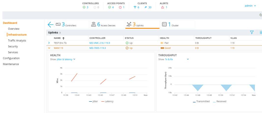
Figure 49 Details Page
